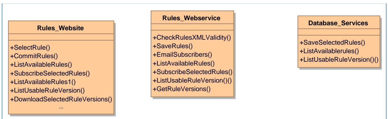
Figure 5: Main Service Class Methods
