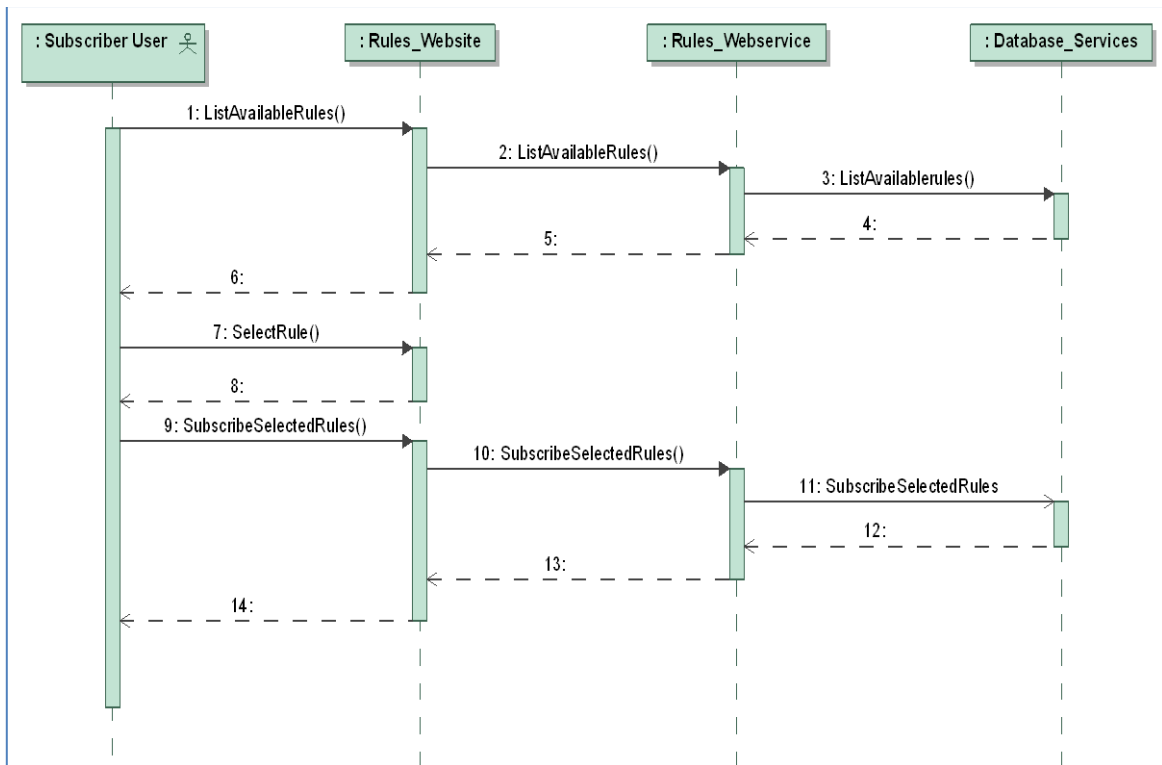
Figure 3: Subscribing to Rules' versions
