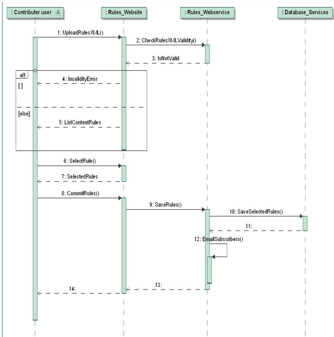
Figure 4: Upload new rules
